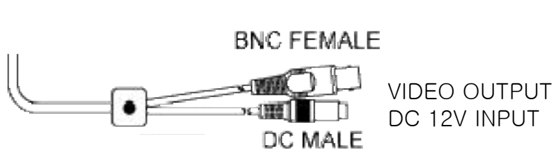
Standard Connection
